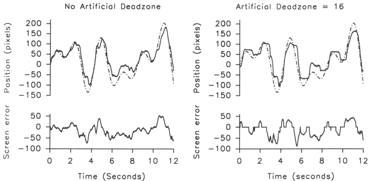
FIGURE 2. Typical human tracking of the pseudorandom waveform (Subject 1, target period = 15 s, manipulation gain = 100%, viewing distance = 50 cm). The records on the left are from a trial with no artificial deadzone; those on the right, with an artificial deadzone of 16 pixels. The top traces show target (broken line) and manipulandum position (solid line) in pixels. The bottom traces show the error that would be displayed on screen. The effect of the large ADZ can be seen easily in the bottom right, where the displayed error is frequently zero despite an obvious positional error between manipulandum and target (upper graph).
