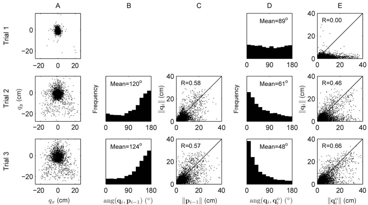
Figure 3. Analysis of hand positions across the trials of a transformation batch. Column A shows the distribution (across all subjects and sessions) of the ‘target-hand vector’ representing the position of the hand relative to the target, \mathbf{q}_i = \mathbf{h}_i - \mathbf{t}_i , separately for trials 1, 2 & 3 of a transformation batch. Columns B and C show the relation between the target-hand vector and the ‘perturbation vector’ from hand to cursor on the previous trial, \mathbf{p}_{i-1} = \mathbf{v}_{i-1} - \mathbf{h}_{i-1} . Column B gives the distribution of the angle between the two vectors, and Column C plots the lengths of the vectors against each other. Columns D and E make the same comparisons between the target-hand vector and the target-hand vector that would place the cursor on the target, \mathbf{q}_i^0 = \mathbf{T}^{-1}\mathbf{t}_i - \mathbf{t}_i . Column D gives the distribution of the angle between the two vectors, and Column E plots the lengths of the vectors against each other. doi:10.1371/journal.pcbi.1001112.g003
