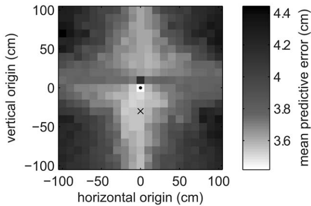
Figure 8. Comparison of possible linear transformation origins for the Bayesian observer model. For each small square the shading denotes the performance of the standard Bayesian observer model when the origin of the linear transformations is set to the centre of that square. Performance is measured using the error between modelled and measured second-trial hand positions, averaged within an experimental session for one subject (after capping all errors at 20 cm) and then averaged across all subjects and all sessions. The small circle shows the start point of the reaches, which is used as the origin in all other modelling. The cross shows the approximate position of the eyes (0, -30 cm). doi:10.1371/journal.pcbi.1001112.g008
