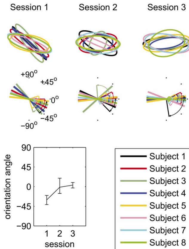
Figure 6. Evolution of the b-c relationship. The top line shows the best fits in each of the experimental sessions, for each of the eight subjects; the middle line shows means and confidence limits on the covariance orientation angles. The bottom-left graph shows the mean across subjects of the orientation angles from the best fits to each subject's data, with 95% confidence limits on the mean found by bootstrapping. doi:10.1371/journal.pcbi.1001112.g006
