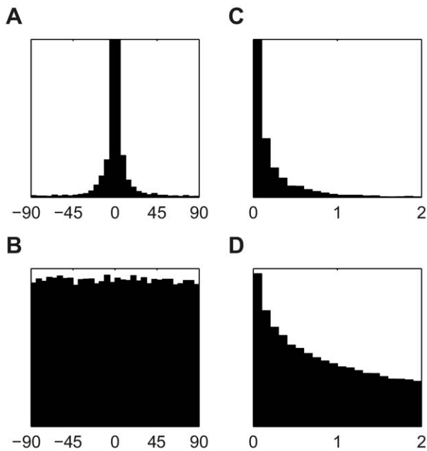
Figure 9. Model validation. (A) The distribution of the difference in covariance orientation angle between pairs of elements in the generating and fitted priors, aggregated across all six pairings of elements. (B) The corresponding distribution when random priors are compared. (C) The distribution of the absolute difference in correlation coefficient between pairs of elements in the generating and fitted priors, aggregated across all six pairings of elements. (D) The corresponding distribution when random priors are compared. doi:10.1371/journal.pcbi.1001112.g009
