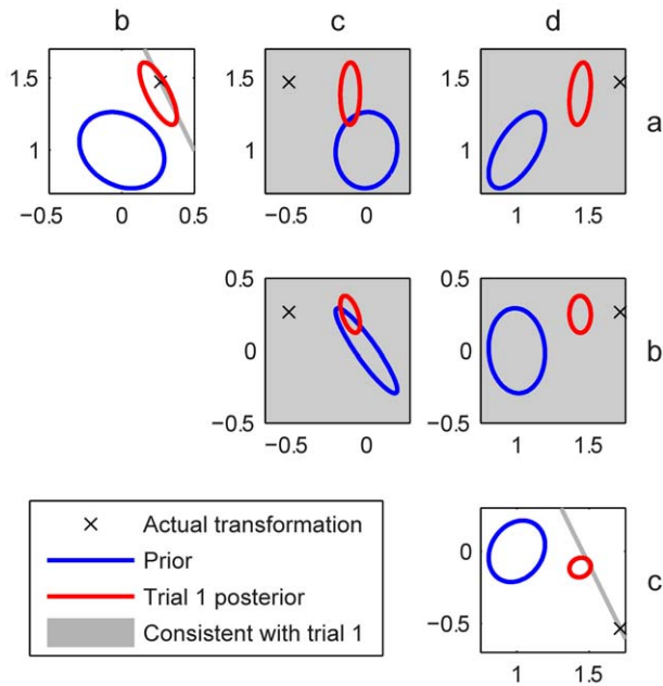
Figure 4. Schematic of the Bayesian observer model. The plots show six 2-dimensional views of the 4-dimensional probability space of the a , b , c & d parameters of the transformation matrix. The Gaussian prior is shown in blue (marginalised 1 s.d. isoprobability ellipses). On the first trial the evidence the subject receives (for simplicity shown here as noiseless) does not fully specify the transformation uniquely, and the transformations consistent with this evidence are shown in gray. This evidence (as a likelihood) is combined with the prior to give the posterior after the first trial (red ellipses: these are shown calculated from the noisy visual feedback) and the MAP of this posterior is taken as the estimate of the transformation. The cross shows the position of the actual transformation matrix used in generating the first-trial evidence. doi:10.1371/journal.pcbi.1001112.g004
