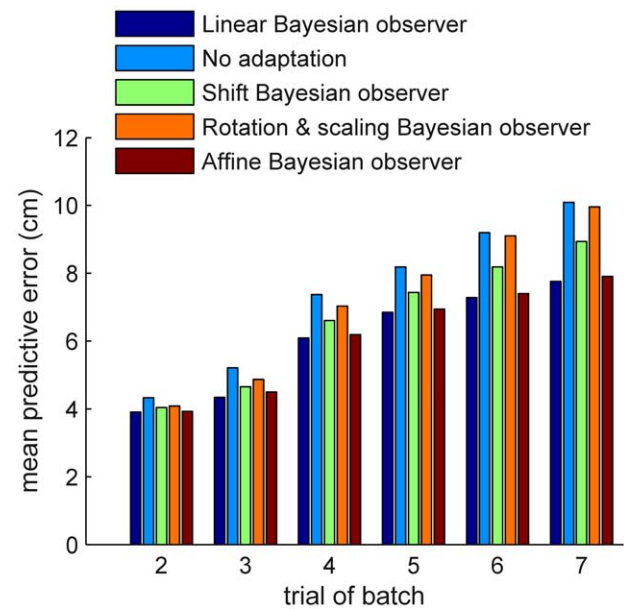
Figure 7. Comparison of standard linear model against other plausible models. Models are compared on the basis of their mean error, across subjects and sessions, in predicting subjects' hand positions on trials 2-7 of transformation batches. For each trial, all batches that lasted for at least that number of trials are used. Errors are capped at 20 cm before averaging, to reduce the effect of outliers. Trial 2 values are computed using 10-fold cross-validation, and later trial values are computed using fits to all transformation batches. doi:10.1371/journal.pcbi.1001112.g007
